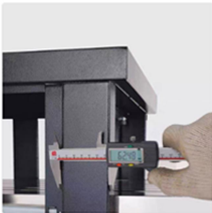
The tool cabinet uses 60mm square columns.
